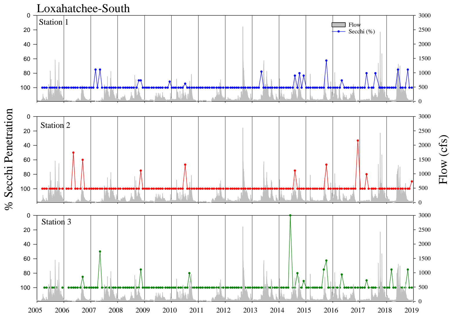
Figure A15. Monthly percent Secchi penetration recorded from 2005 – 2018 at Loxahatchee-South Station 1 (top), Station 2 (middle) and Station 3 (bottom) and the sum of the mean daily flow rate at the Lainhart Dam and S46 structures as recorded by the U.S. Geological Survey and the South Florida Water Management District.
