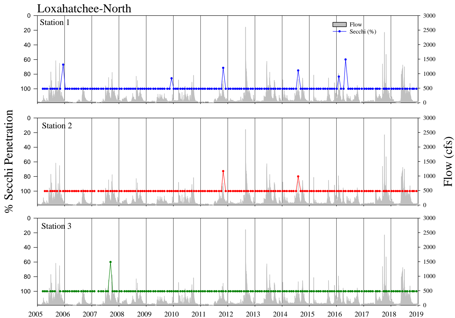
Figure A14. Monthly percent Secchi penetration recorded from 2005 – 2018 at Loxahatchee-North Station 1 (top), Station 2 (middle) and Station 3 (bottom) and the sum of the mean daily flow rate at the Lainhart Dam and S46 structures as recorded by the U.S. Geological Survey and the South Florida Water Management District.
