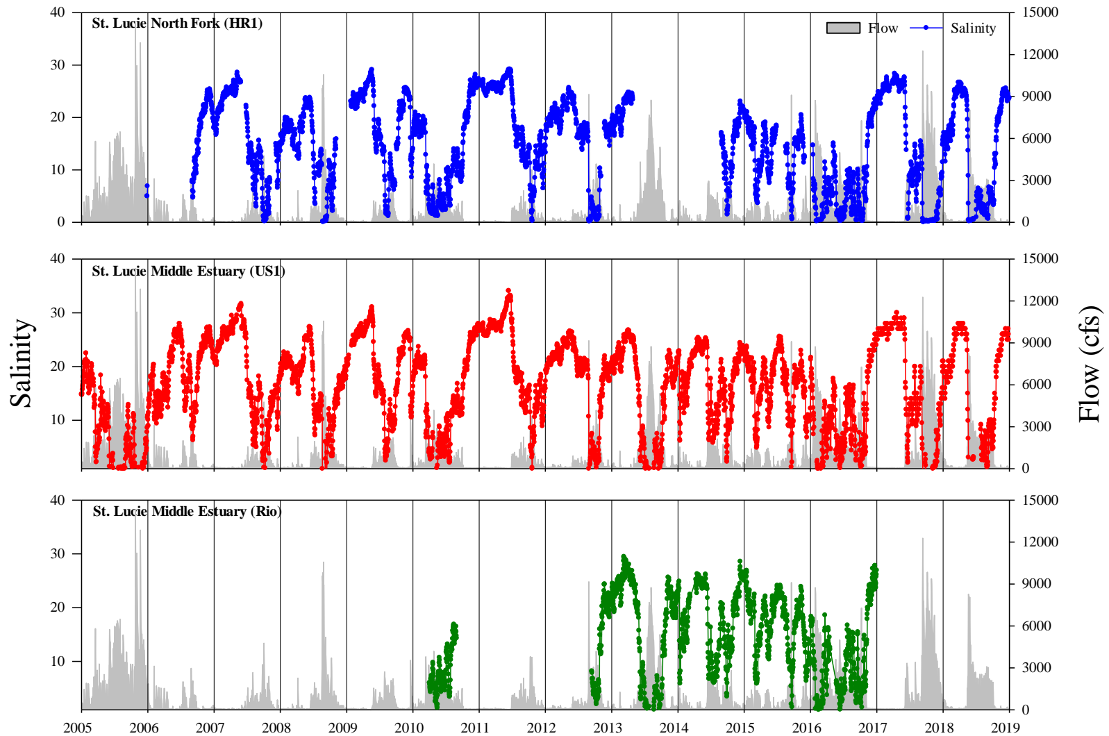
Figure A3. Mean daily salinity recorded by continuous data loggers from 2005 – 2018 at the St. Lucie North Fork HR1 (top), St. Lucie US1 Roosevelt Bridge (middle) and St. Lucie middle estuary Rio (bottom) stations and the sum of the mean flow rate at the S80, S97, S49 and Gordy structures. Salinity and flow data from the U.S. Geological Survey and the South Florida Water Management District.
