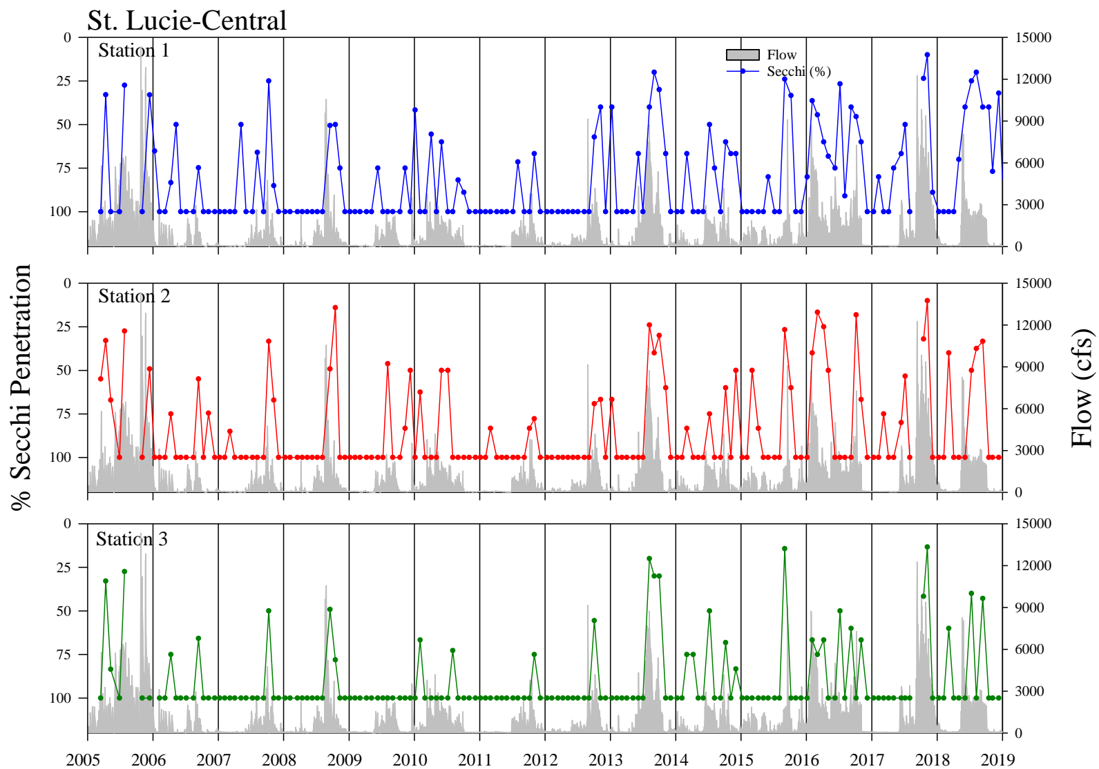
Figure A13. Monthly percent Secchi penetration recorded from 2005 – 2018 at St. Lucie-Central Station 1 (top), Station 2 (middle) and Station 3 (bottom) and the sum of the mean daily flow rate at the S80, S97, S49 and Gordy structures as recorded by the South Florida Water Management District.
