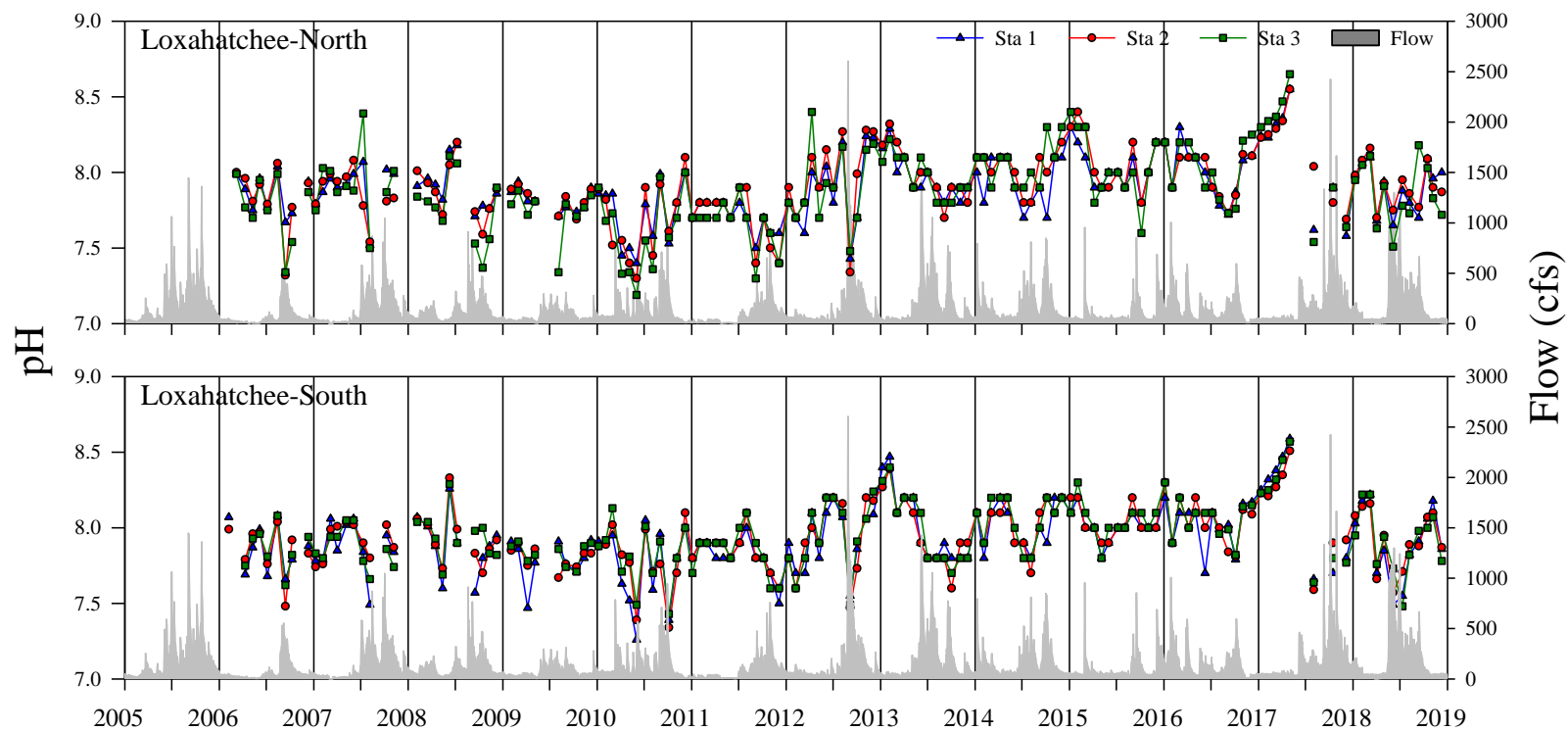
Figure A10. Monthly pH recorded at stations from 2006 – 2018 in the Loxahatchee-North (top) and Loxahatchee-South (bottom) study sites and the sum of the mean daily flow rate at the Lainhart Dam and S46 structures as recorded by the U.S. Geological Survey and the South Florida Water Management District.
