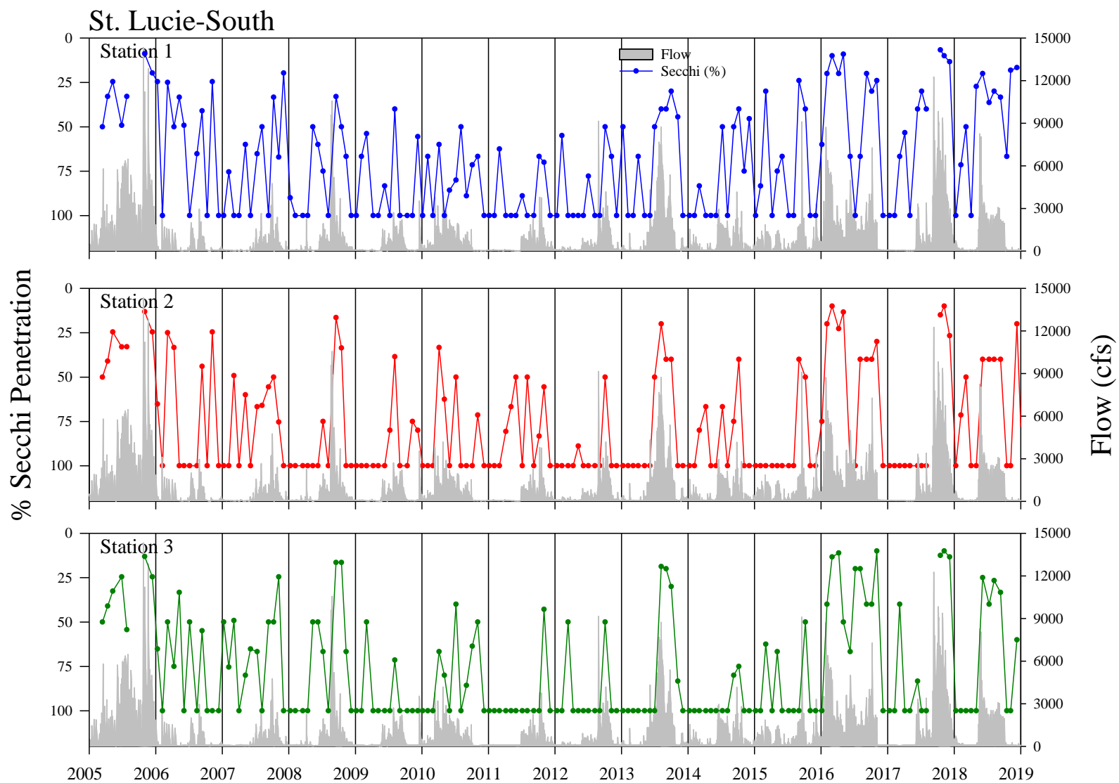
Figure A12. Monthly percent Secchi penetration recorded from 2005 – 2018 at St. Lucie-South Station 1 (top), Station 2 (middle) and Station 3 (bottom) and the sum of the mean daily flow rate at the S80, S97, S49 and Gordy structures as recorded by the South Florida Water Management District.
