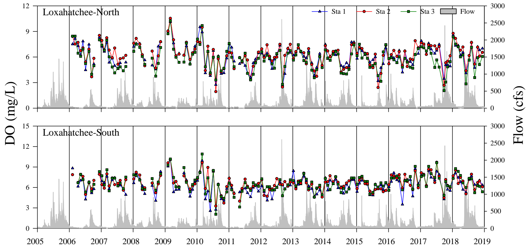
Figure A8. Monthly dissolved oxygen concentration recorded at stations from 2006 – 2018 in the Loxahatchee-North (top) and Loxahatchee-South (bottom) study sites and the sum of the mean daily flow rate at the Lainhart Dam and S46 structures as recorded by the U.S. Geological Survey and the South Florida Water Management District.
