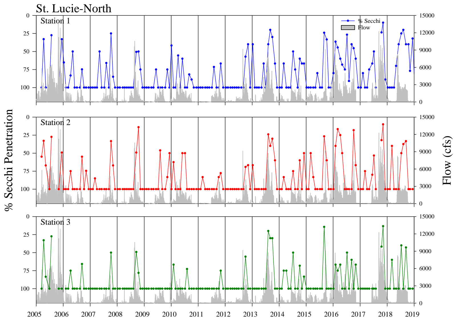
Figure A11. Monthly percent Secchi penetration recorded from 2005 – 2018 at St. Lucie-North Station 1 (top), Station 2 (middle) and Station 3 (bottom) and the sum of the mean daily flow rate at the S80, S97, S49 and Gordy structures as recorded by the South Florida Water Management District.
