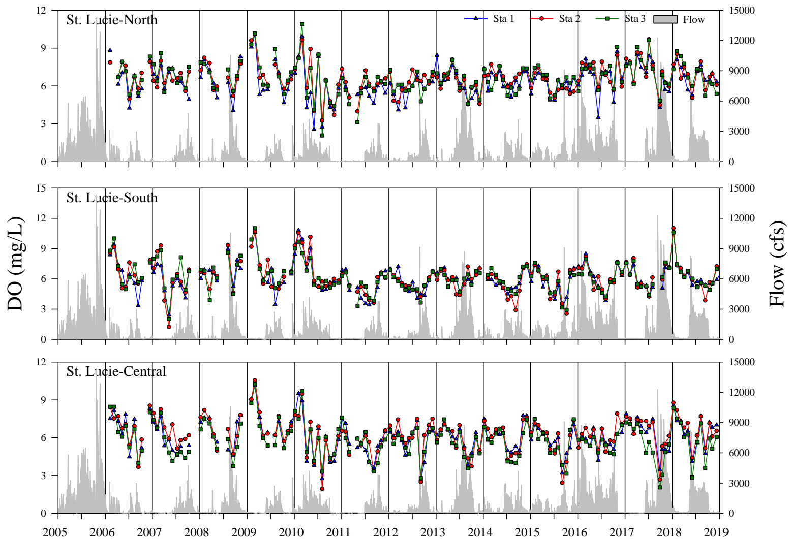
Figure A7. Monthly dissolved oxygen concentration recorded at stations from 2006 – 2018 in the St. Lucie-North (top), St. Lucie-South (middle) and St. Lucie-Central (bottom) study sites and the sum of the mean flow rate at the S80, S97, S49 and Gordy structures as recorded by the South Florida Water Management District.
