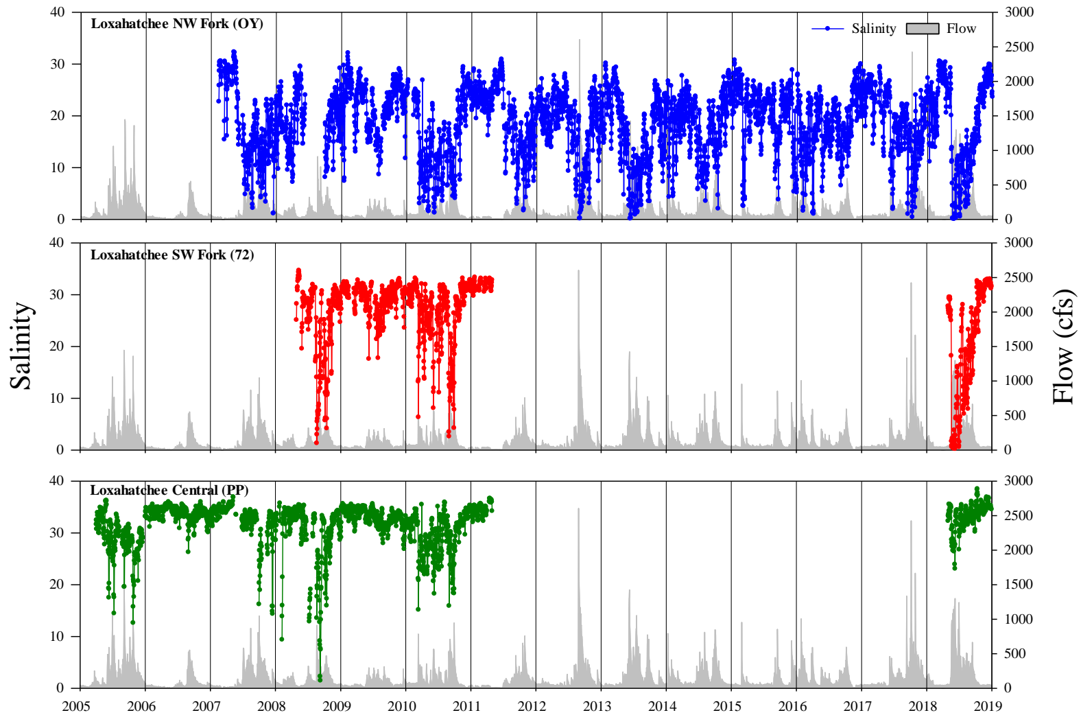
Figure A4. Mean daily salinity recorded by continuous data loggers from 2005 – 2018 at the Loxahatchee NW Fork OY (top), Loxahatchee SW Fork 72 (middle) and Loxahatchee central estuary PP (bottom) stations and the sum of the mean flow rate at the Lainhart Dam and S46 structures. Salinity data from the Loxahatchee River District and flow data from the U.S. Geological Survey and the South Florida Water Management District.
