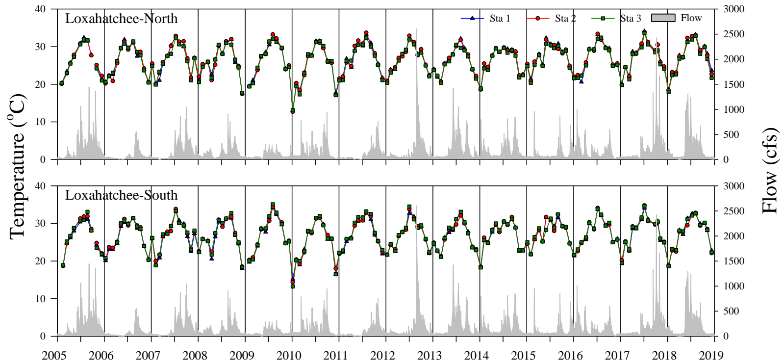
Figure A6. Monthly water temperature recorded at stations from 2005 – 2018 in the Loxahatchee-North (top) and Loxahatchee-South (bottom) study sites and the sum of the mean daily flow rate at the Lainhart Dam and S46 structures as recorded by the U.S. Geological Survey and the South Florida Water Management District.
