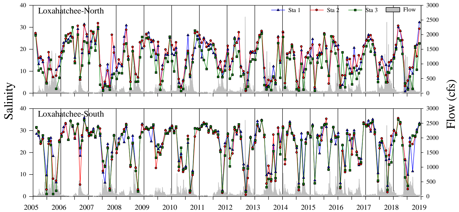
Figure A2. Monthly salinity recorded at stations from 2005 – 2018 in the Loxahatchee-North (top) and Loxahatchee-South (bottom) study sites and the sum of the mean daily flow rate at the Lainhart Dam and S46 structures as recorded by the U.S. Geological Survey and the South Florida Water Management District.
