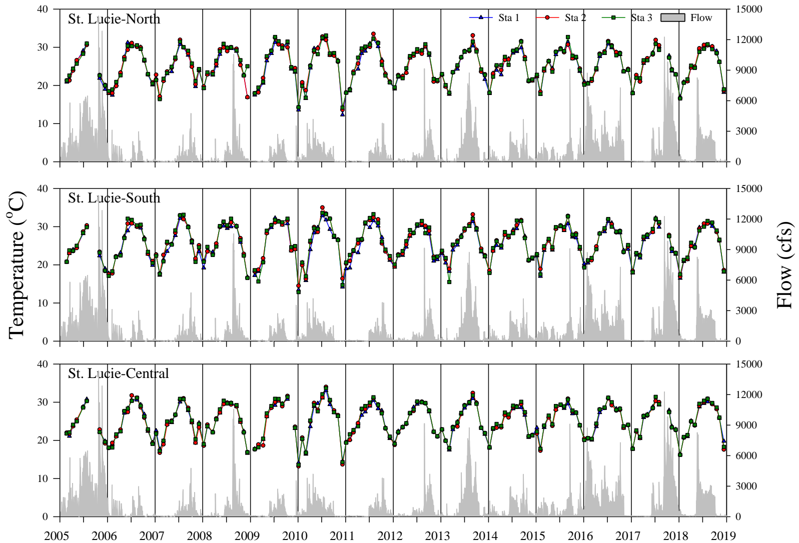
Figure A5. Monthly water temperature recorded at stations from 2005 – 2018 in the St. Lucie-North (top), St. Lucie-South (middle) and St. Lucie-Central (bottom) study sites and the sum of the mean flow rate at the S80, S97, S49 and Gordy structures as recorded by the South Florida Water Management District.
