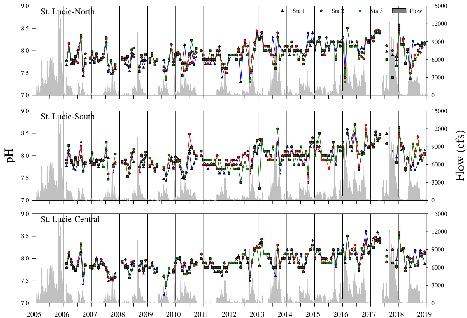
Figure A9. Monthly pH recorded at stations from 2006 – 2018 in the St. Lucie-North (top), St. Lucie-South (middle) and St. Lucie-Central (bottom) study sites and the sum of the mean flow rate at the S80, S97, S49 and Gordy structures as recorded by the South Florida Water Management District.
