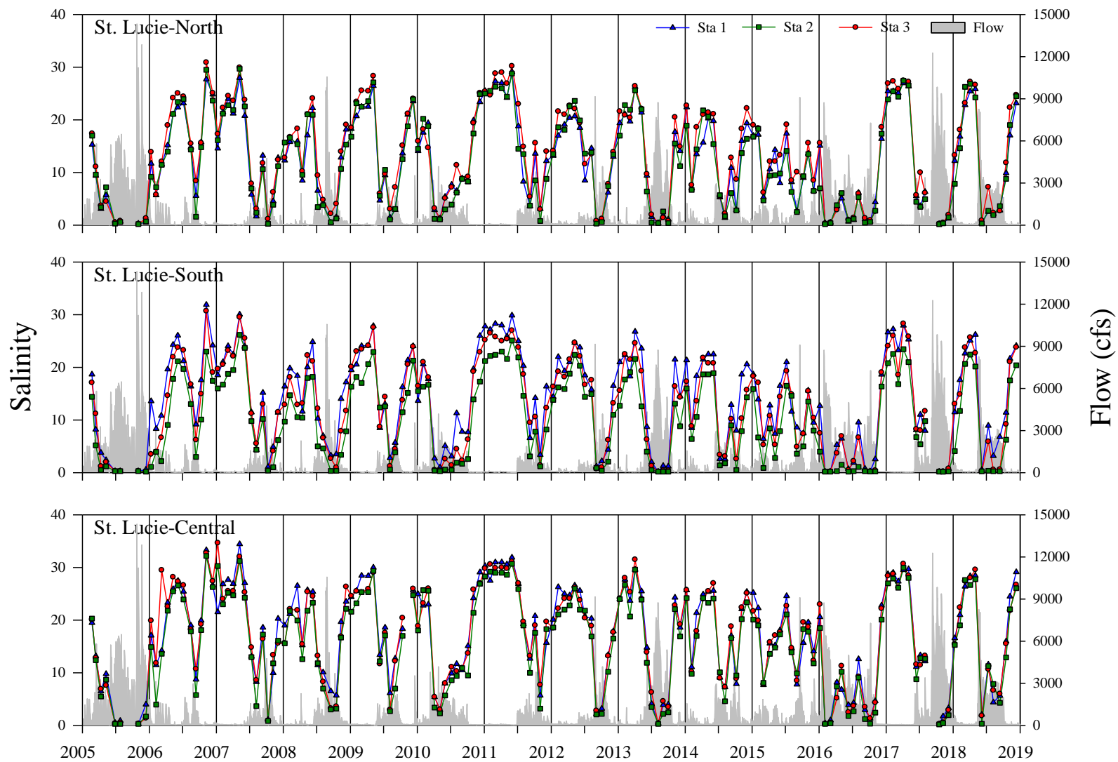
Figure A1. Monthly salinity recorded at stations from 2005 – 2018 in the St. Lucie-North (top), St. Lucie-South (middle) and St. Lucie-Central (bottom) study sites and the sum of the mean flow rate at the S80, S97, S49 and Gordy structures as recorded by the South Florida Water Management District.
