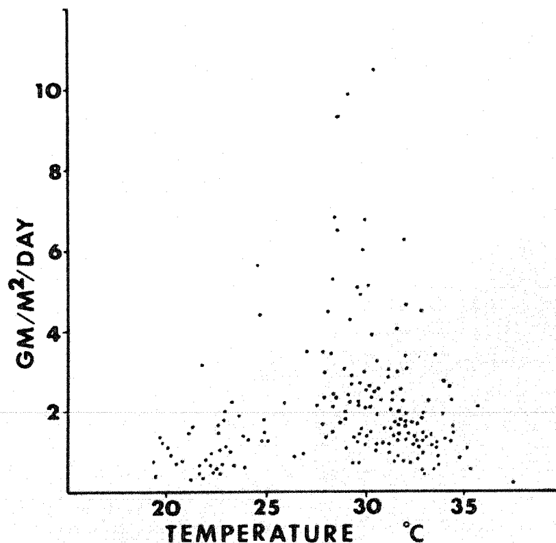
Figure 6. Response of Thalassia production to temperature in south Florida.
