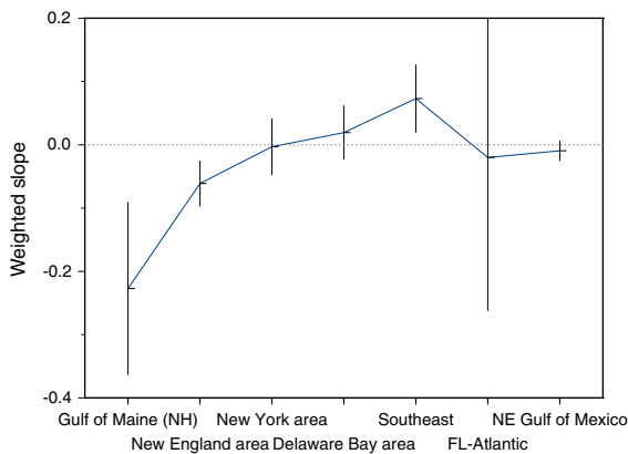
Fig. 4 Weighted slope with 90% confidence bars from meta analyses of multiple datasets from New Hampshire (NH) in the Gulf of Maine region to the Northeast (NE) Gulf of México region with time series spanning different years. A weighted slope was an average of dataset-specific slopes weighted inverse to mean square error, which accounts for variability. Regions and areas with regions are described in the text and in Fig. 1. The datasets were grouped and oriented generally north to south on the x-axis. The datasets from Gulf of Maine New Hampshire are from the Great Bay. The New England, New York, and Delaware Bay constitute areas within the Mid-Atlantic region. The Southeast, Florida Atlantic, and Northeast Gulf are separate regions
