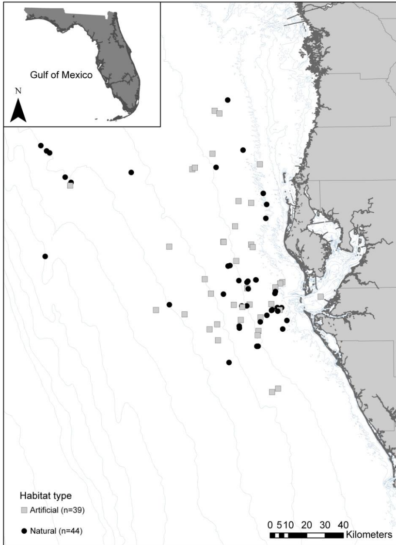
Fig. 1. Study area and sites surveyed for goliath grouper between October 2007 and May 2010. Surveys took place during all months of the year over artificial and natural habitat that ranged in depth from 7 – 48 m.
