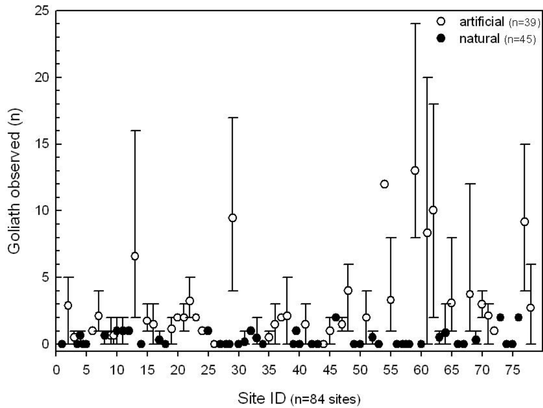
Fig. 9. Number of goliath grouper observed at each site during the study period (October 2007 – May 2010). Symbols represent mean abundance and error bars designate the maximum and minimum number observed at each site. Sites are numbered in order of decreasing latitude (i.e., site 1 is the northernmost site). Total number of surveys = 378.
