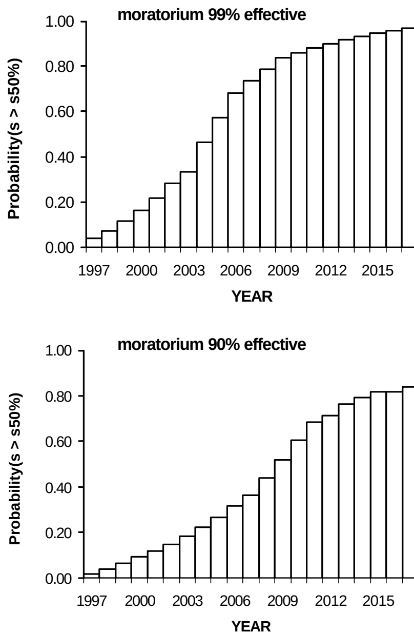
Figure 10. Probability stock will recover to spawning biomass levels corresponding to a 50 percent SPR assuming the moratorium on harvest is 99 percent effective (top panel) or 90 percent effective (bottom panel) (Porch, 2004).
